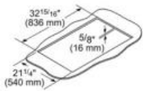
Cutout for insert without liner accessory
