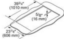
Cutout for insert with liner accessory LINER236
